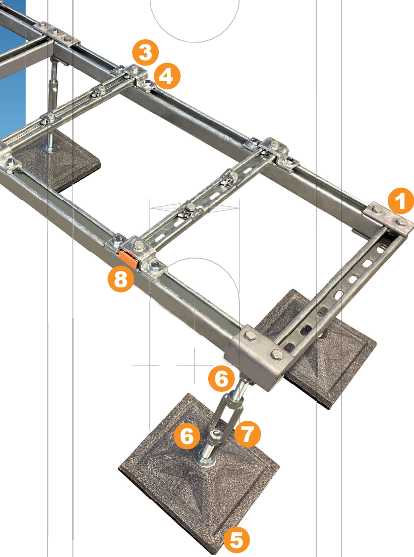
PROLINK AYAK UZATMA ELEMANI PROLINK BASE EXTENSIONS
